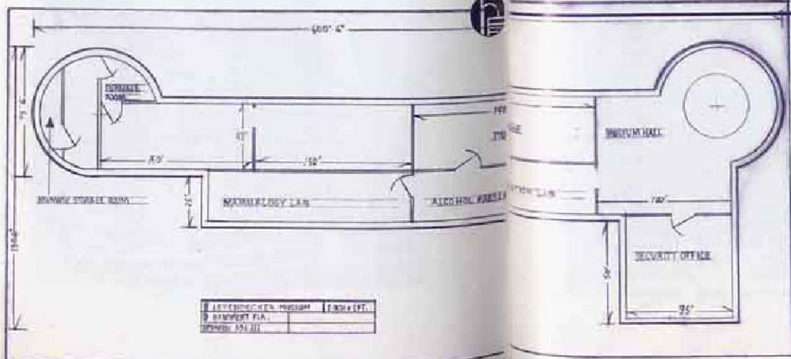
Blueprints for the original Leyendecker basement.
