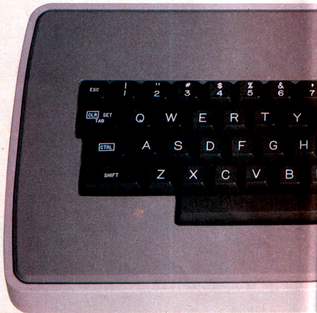
The Screenonics "Sidewriter" outboard keyboard sits atop the original Atari 400 computer
