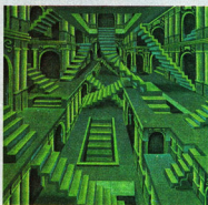
1 Gameboard Map
