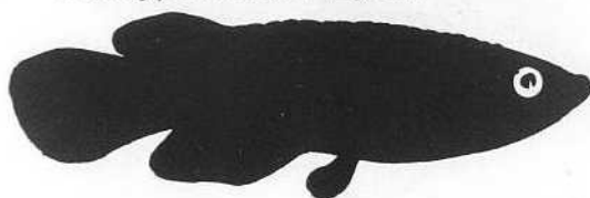
Playfair's Panchax Pachypanchax Playfairi
