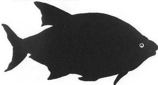
Bream Abramis Brama
