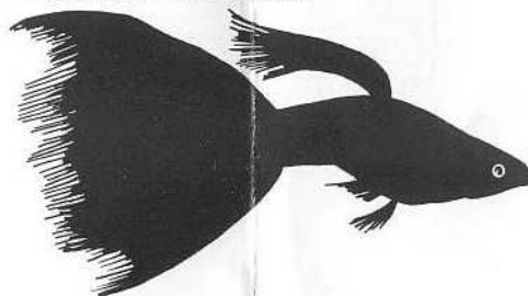
Guppy Poecilia Reticulata
