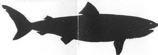
Basking Shark Cetorhinus maximus
