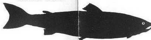
Salmon Salmo Salar
